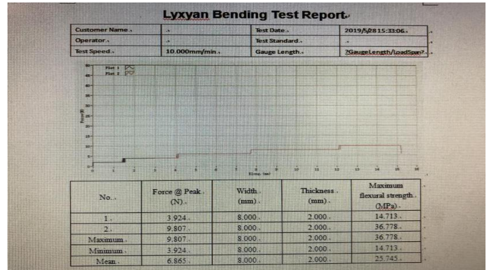
Test Curve
